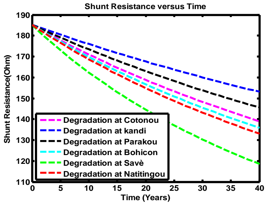
Fig. 9. Shunt resistance degradation
