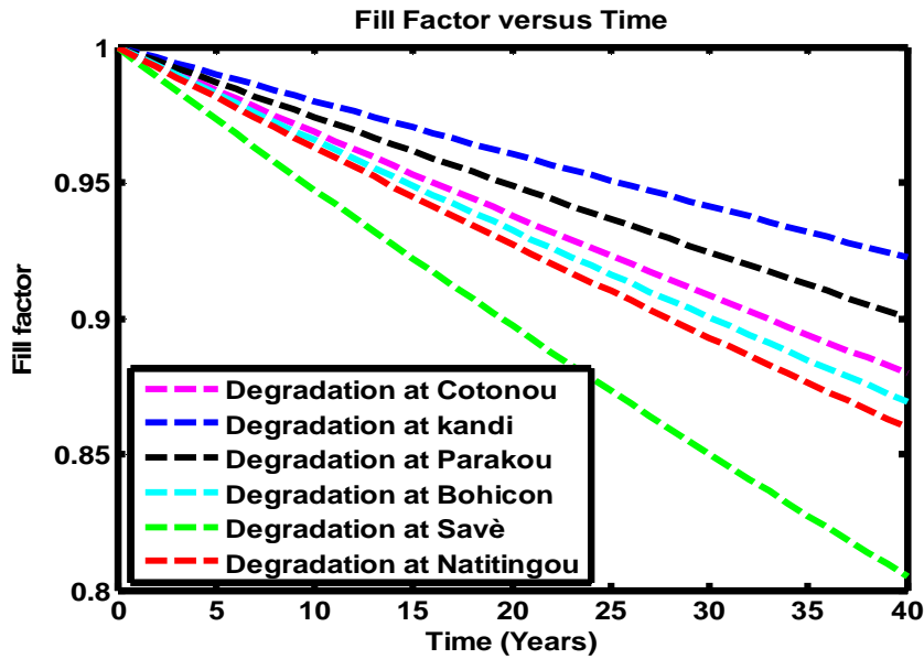
Fig.11. Fill Factor degradation
