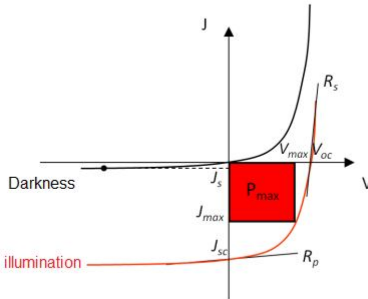
Figure 7: I-V characteristics under darkness and under AM1.5 lighting [50]
