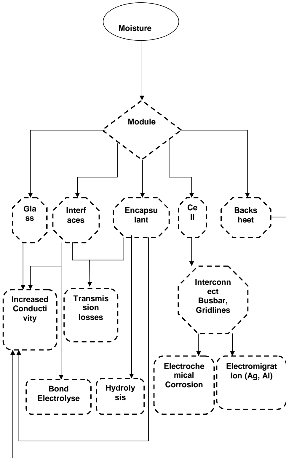
Fig. 5. Effects of moisture and degradation mechanism [47]
