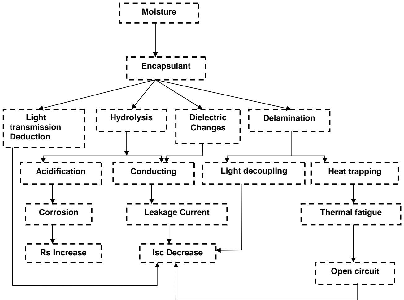
Fig.6. Degradation mechanisms of PV module encapsulant-Impact on module electrical parameters [47]
