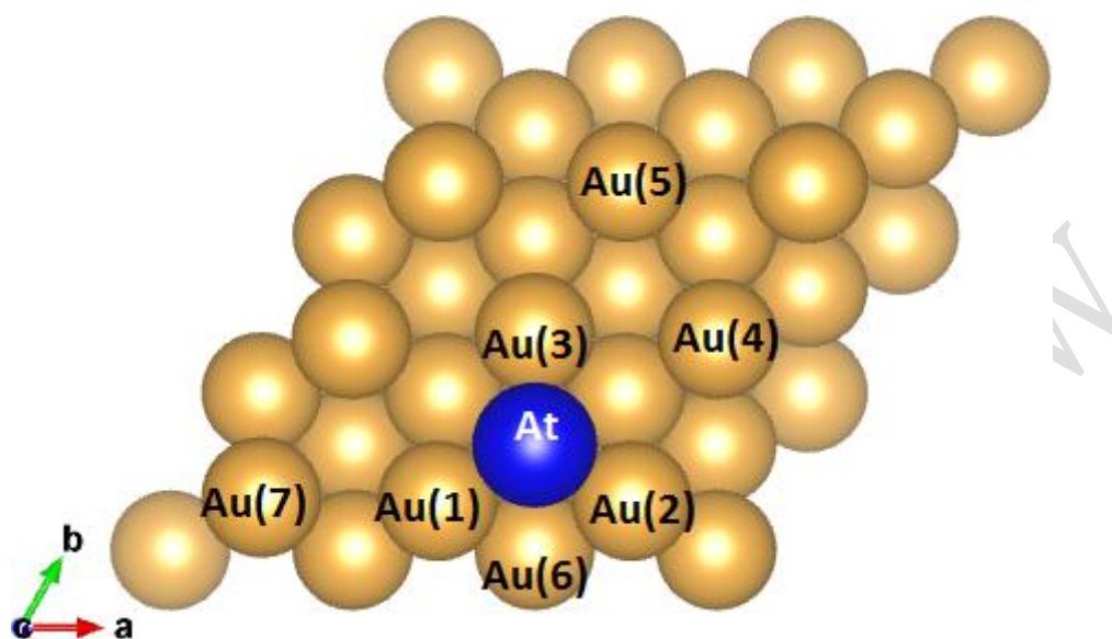
Figure 2. Schematic diagram of At on Au (111) surface.
