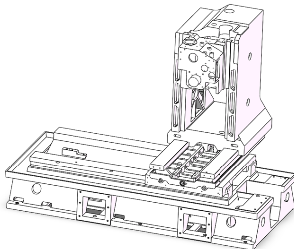
Figure 1 Three-dimensional model diagram of horizontal machining center
