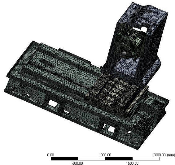
Figure 2 Grid diagram of horizontal machining center
