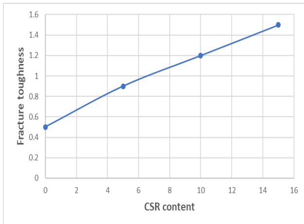
Figure 1. Effect of CSR content on fracture toughness of epoxy resin
