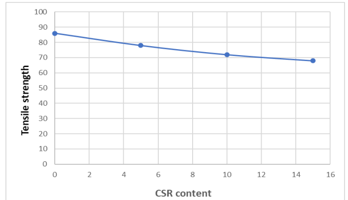
Figure 2. Effect of CSR content on Tensile strength of epoxy resin
