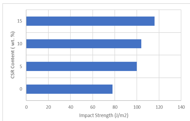
Figure 3. Effect of CSR content on the impact strength of epoxy resin
