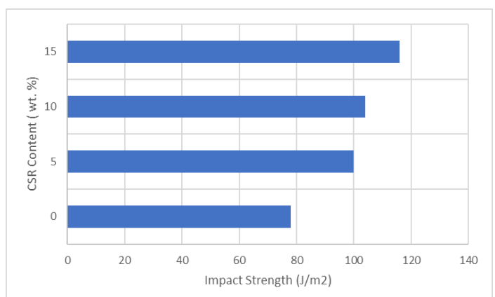
Graph 3: Izod impact test
