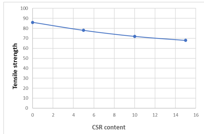
Grapp 1: Tensile strength ratio with CSR content
