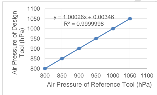
Figure 8. Graf of air pressure parameter calibration.
