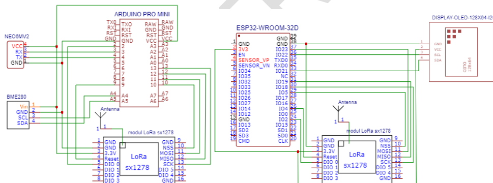
Figure 3. Schematic design
