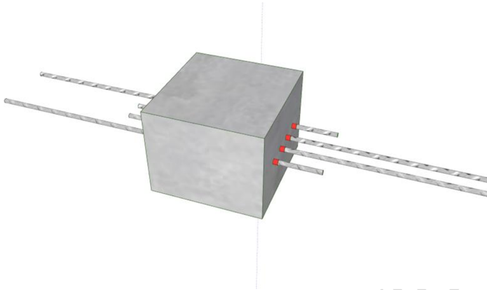
Figure 8: Four rebar lap test[41]
