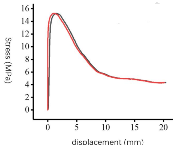
Figure 3. Bonding slip curve [38]
