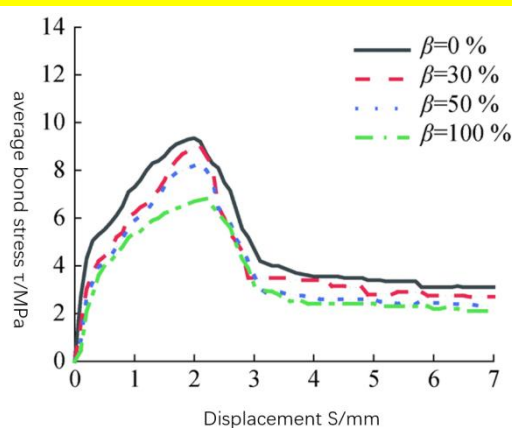
Figure 5. \tau -s curve with different substitution rate \beta for 14mm diameter of steel bar [40]
