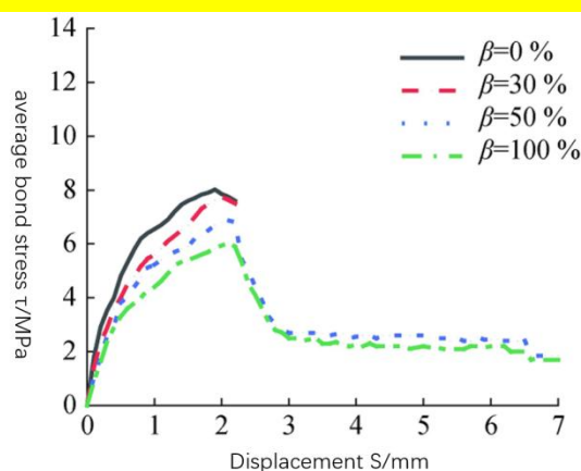
Figure 6. \tau -s curve with different substitution rate \beta for 18mm diameter of steel bar [40]
