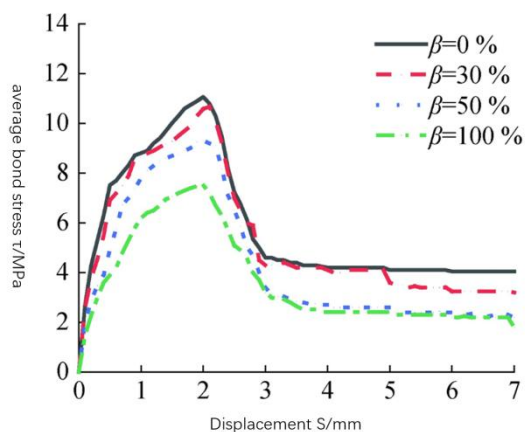
Figure 4. \tau -s curve with different substitution rate \beta for 12mm diameter of steel bar [40]
