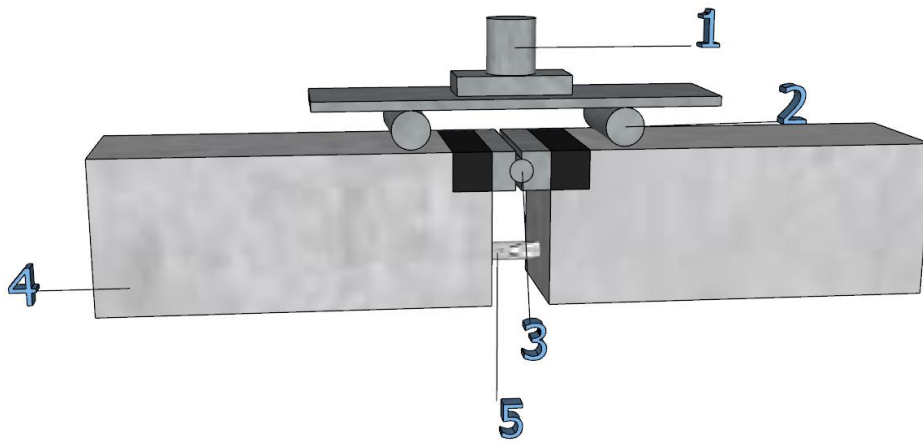
1- Upper loading device 2-Loading distribution point 3-Turning hinge 4-Test block 5-Rebar
