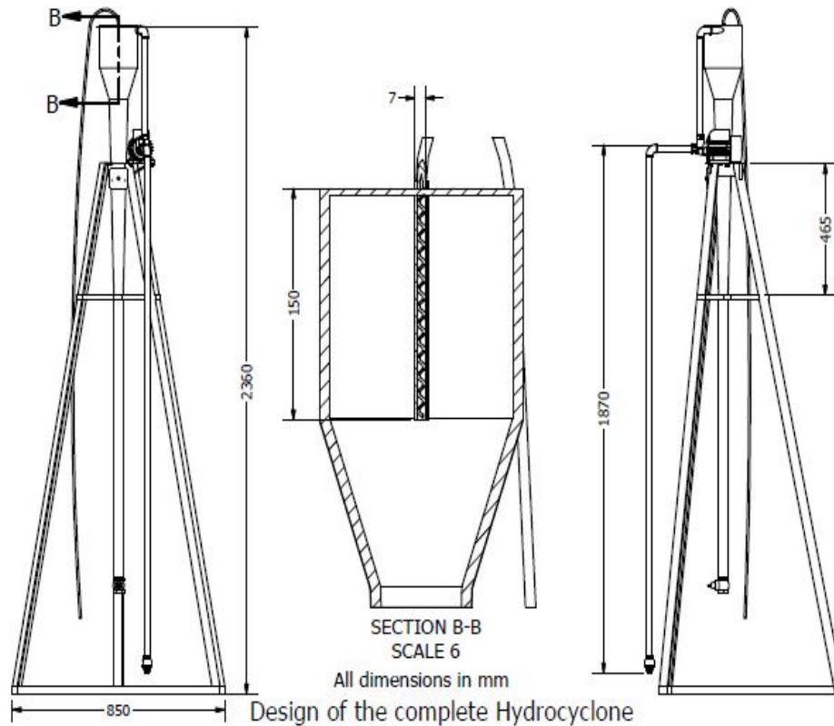
Figure 1: Sectional View of the Designed LLHC
