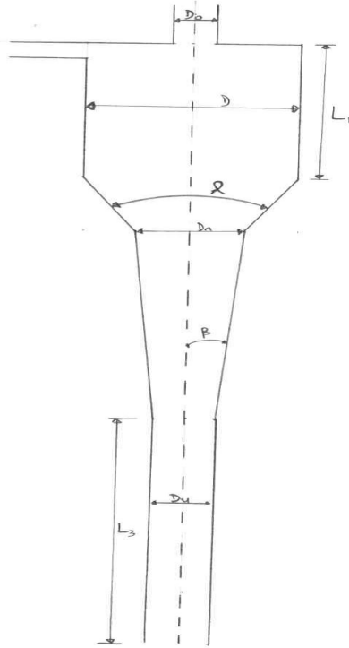
Figure 2: Colman and Thew's hydrocyclone geometry analysis and ration
