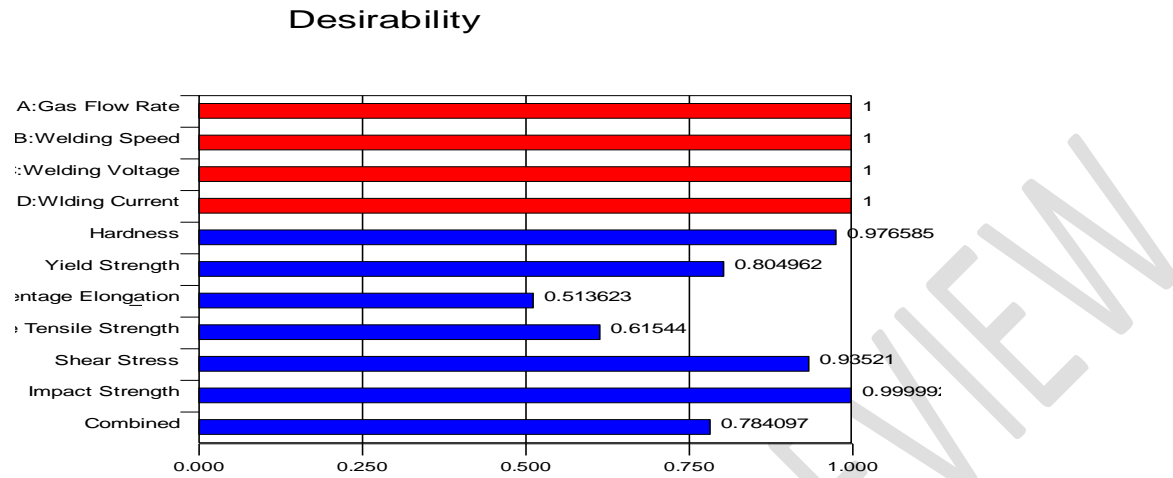
Figure 7.2: The Desirability Plot for the Optimal Solutions
