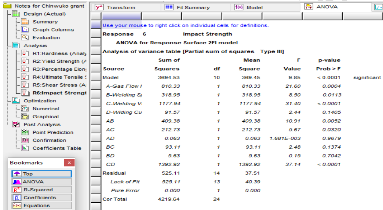
Figure 6.1: Analysis of Variance for the Impact of Energy Modeling
