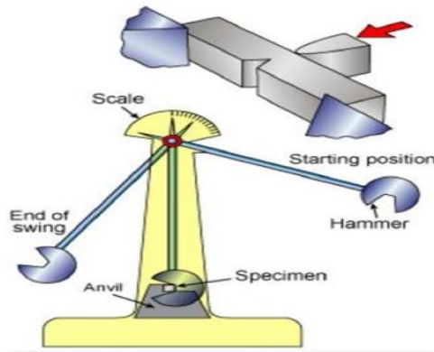
Figure 1b: Impact Energy Testing Machine and its Experimental Specimen
