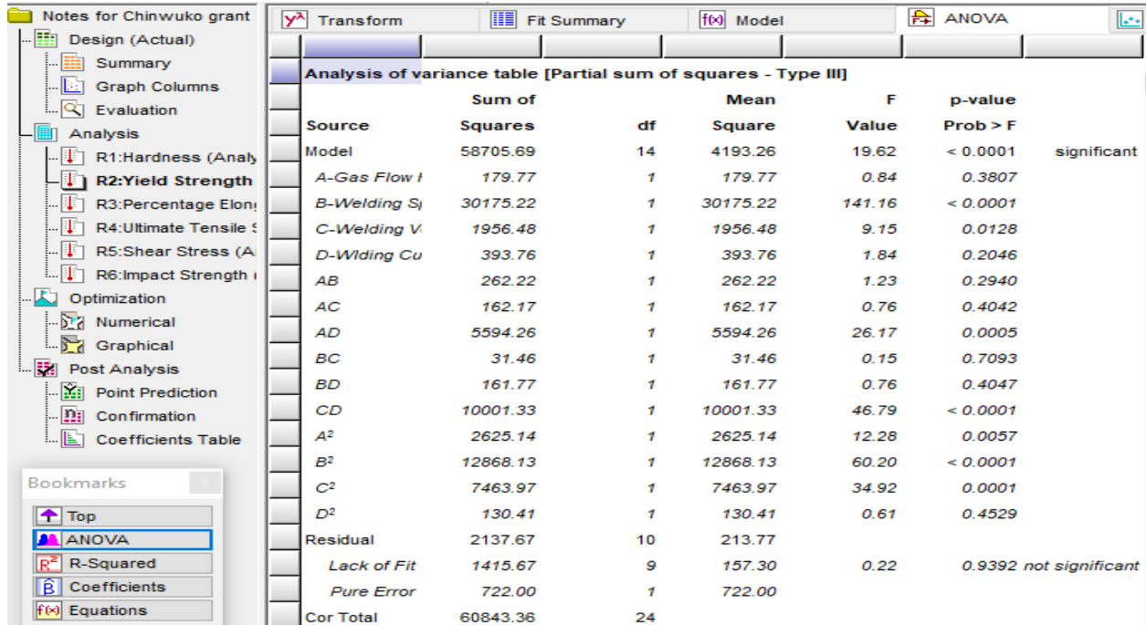
Figure 2.1: Analysis of Variance for the Yield Strength Modeling
