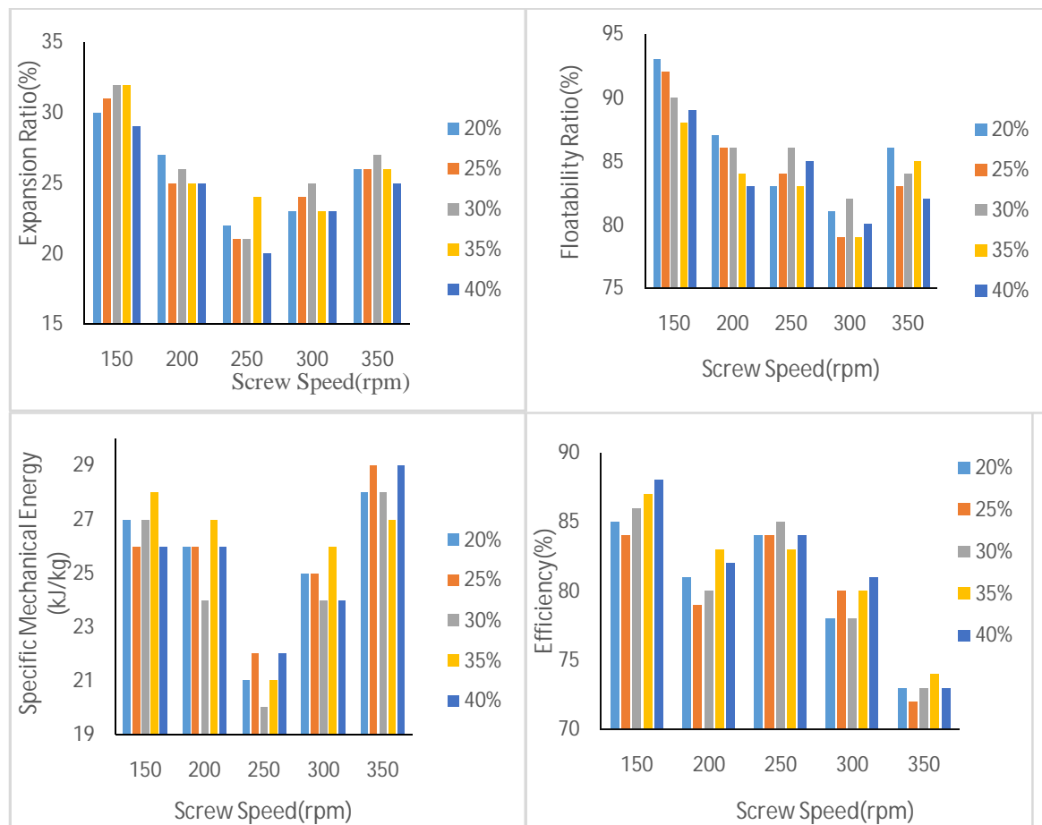
Figure 4 Graphical presentation of effect of screw speed on variables considered
