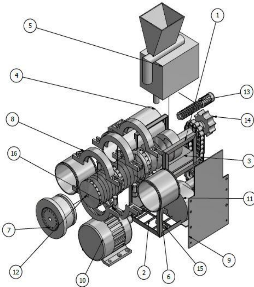
Figure. 1 Extrusion machine and its exploded view
