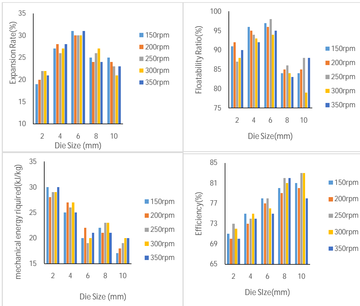
Figure 3 Graphical presentation of effect of die size on variables considered
