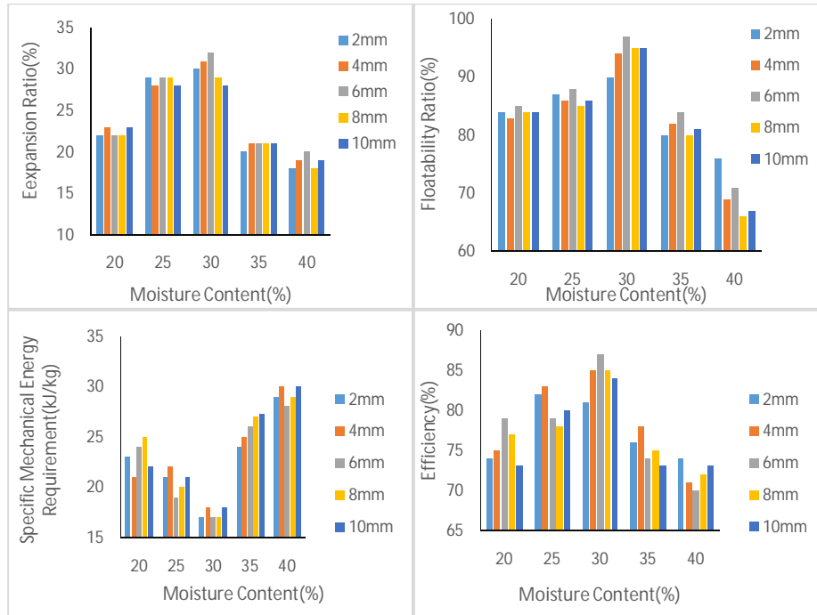
Figure. 2 Graphical presentation of effect of moisture content on variables considered
