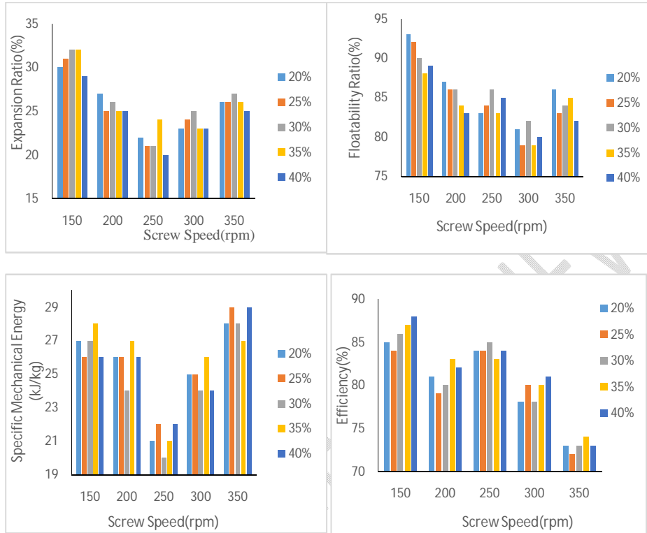
Figure: 4 Graphical presentation of effect of screw speed on variables considered
