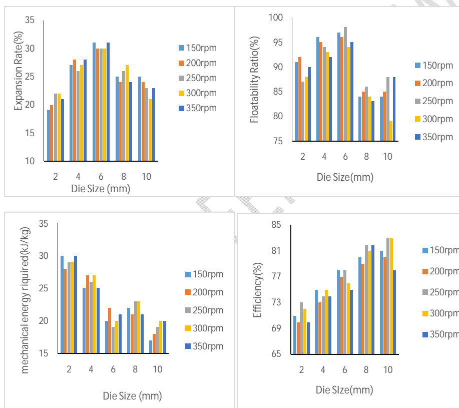
Figure. 3 Graphical presentation of effect of die size on variables considered
