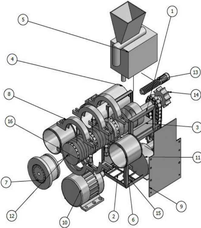
Figure. 1 The Extrusion machine and its exploded view
