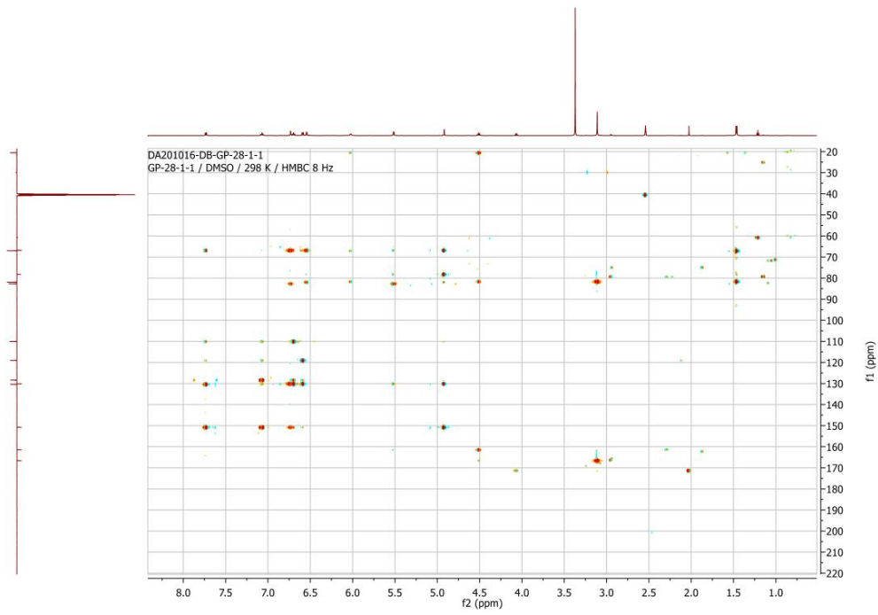
Fig. 6. HMBC spectrum of verticillin D (DMSO-d6)
