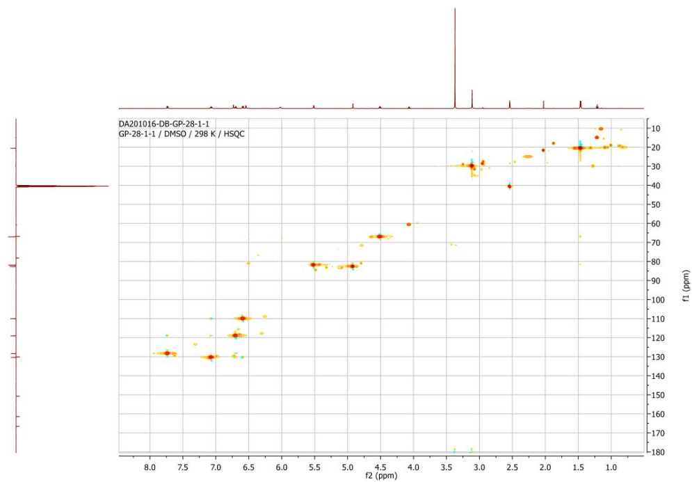
Fig. 5. HSQC spectrum of verticillin D (DMSO-d6)
