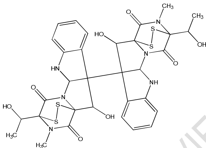
Fig 2: Structure of Verticillin D
