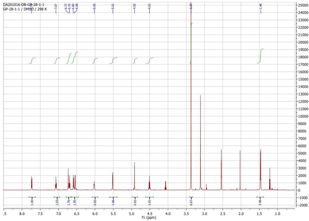
Fig. 2. ^1\text{H} RMN spectrum of verticillin D (DMSO-d 6 )
