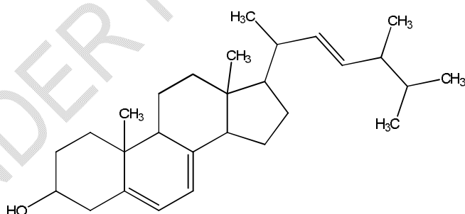
Fig 1: Structure of Ergosterol
