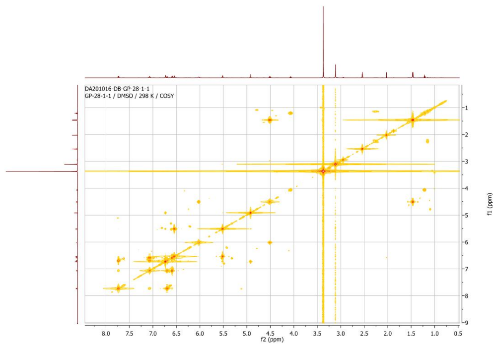
Fig. 4. COSY spectrum of verticillin D (DMSO-d6)
