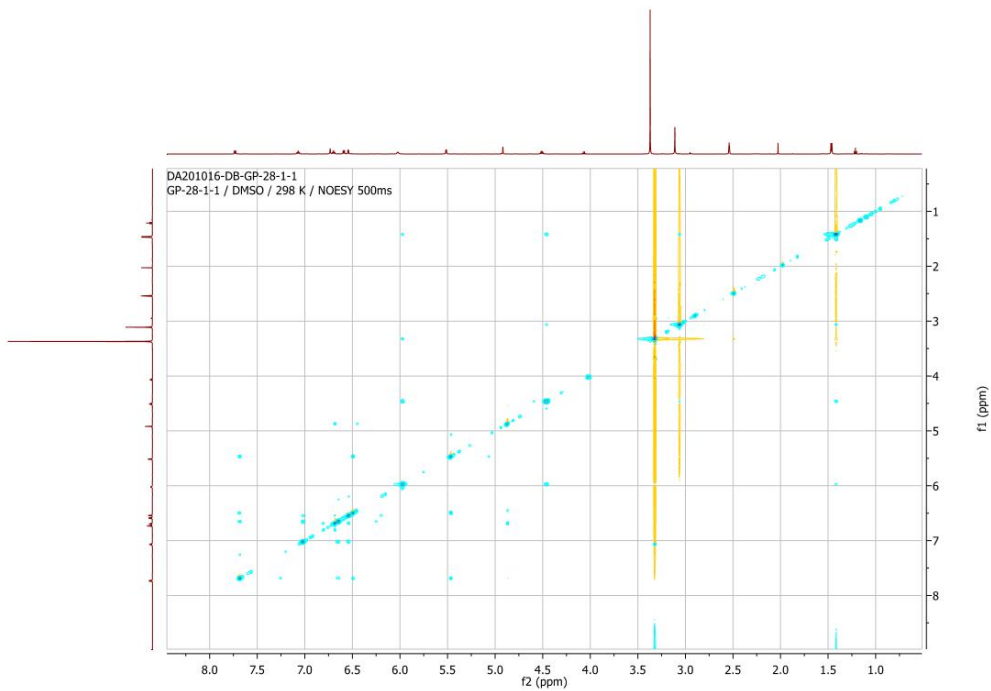
Fig. 7. NOESY spectrum of verticillin D (DMSO-d6)
