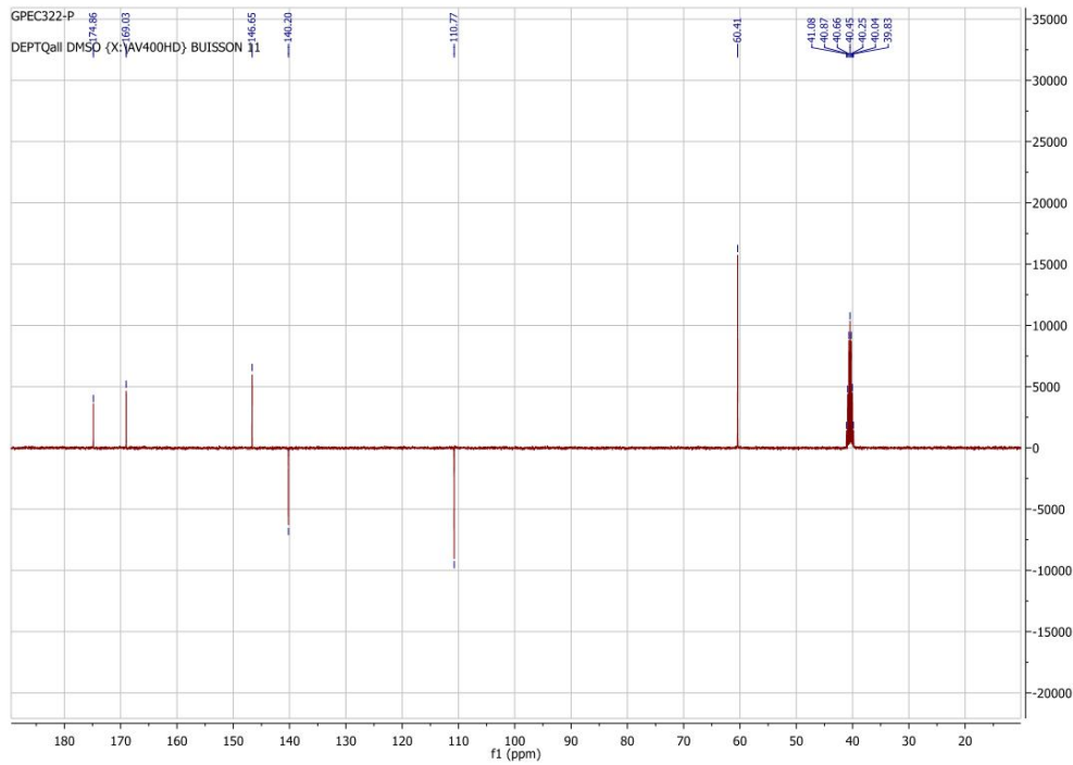
Fig. 3. DEPT Q spectrum of verticillin D (DMSO-d 6 )
