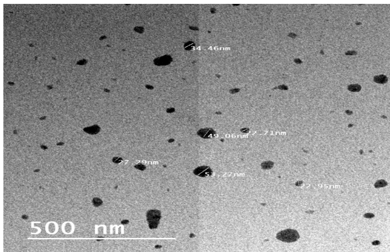
Figure 1: TEM measurements of the nano-metric particle size of the obtained 20:20:20 NPK nano-metric fertilizer.
