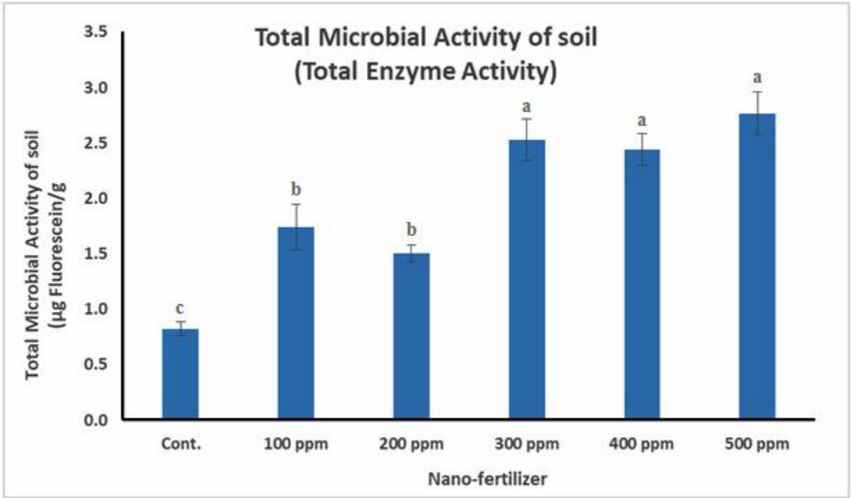
Figure 4: Effect of nano-fertilizer on microbial activity in soil as a result of combined analysis for the 2020 and 2021 seasons. Different letters above the bars indicate significant differences between treatments after one-way ANOVA and L.S.D test ( P \leq 0.05 ).
