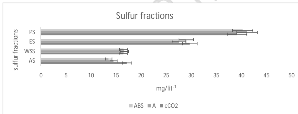
Fig 2. Distribution of sulphur fractions available sulphur(AS), water-solublesulphur(WSS), exchangeablesulphur(ES), and precipitated sulphur(PS) from three different soils elevated, ambient, and ambient bulk soil.
