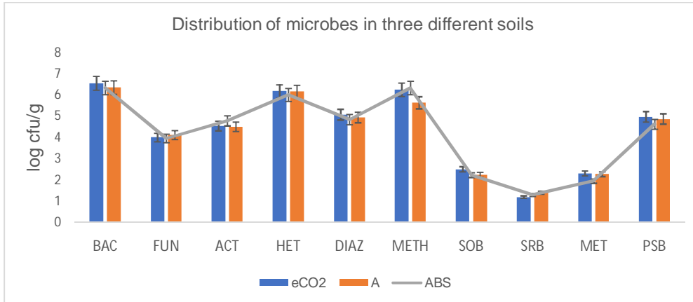
Fig.1. Distribution of different groups of microbes. Bacteria, fungi, actinomycetes, heterotrophs, diazotrophs, methanotrophs, sulphur-oxidizing bacteria, sulphur reducing bacteria, methanogens, and phosphate solubilizing bacteria from three different soils elevated(eCO 2 ), ambient(A), and ambient bulk soil (ABS).
