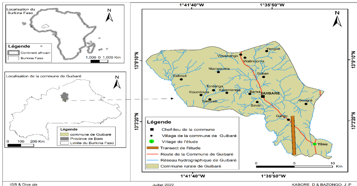
Figure 1. Locality of soils collection
