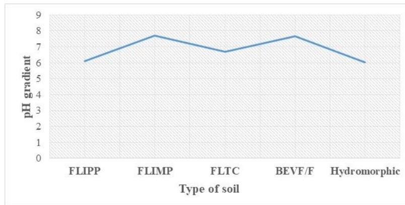
Figure 5. pH water according to soil types
