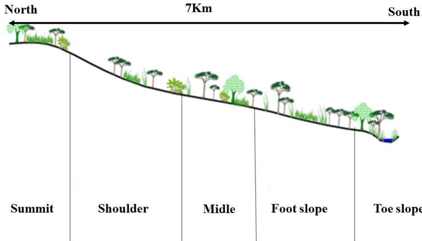
Figure 3. Toposequence in Yilou
