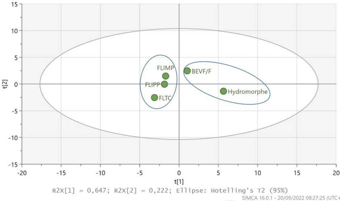
Figure 6. Principal component analysis of the five soils according to the physicochemical parameters
