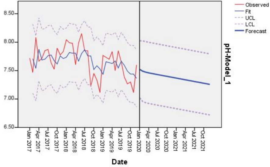
Figure 2: Observed data and ARIMA (1, 1, 1) model prediction of pH
