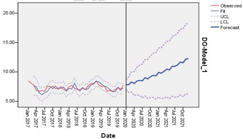
Figure 3: Observed data and ARIMA (2, 2, 5) model prediction of DO mg/l
