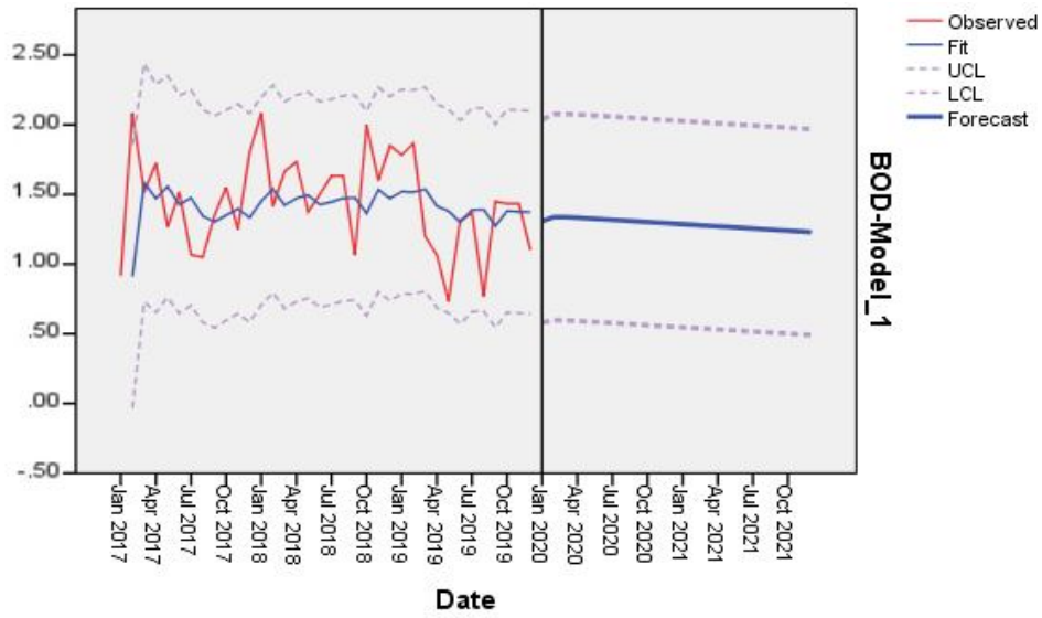
Figure 4: Observed data and ARIMA (1, 1, 1) model prediction of BOD mg/l
