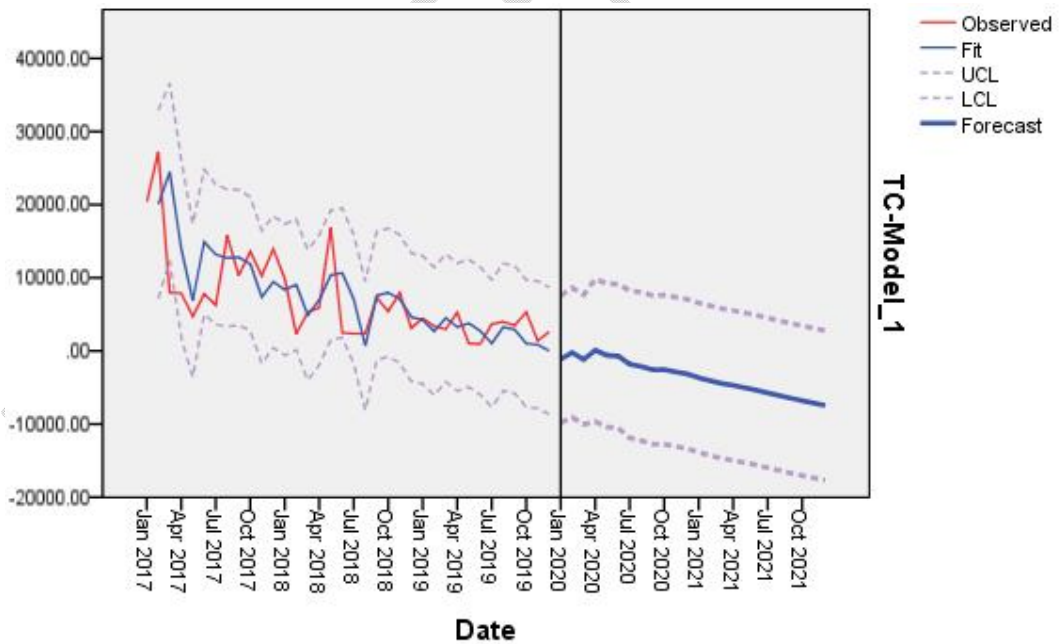
Figure 5: Observed data and ARIMA (3, 1, 1) model prediction of TC MPN/100ml
