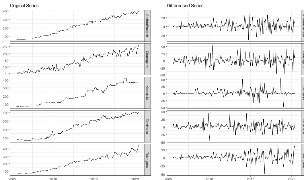
Figure 1. Time plot of the original and differenced series
