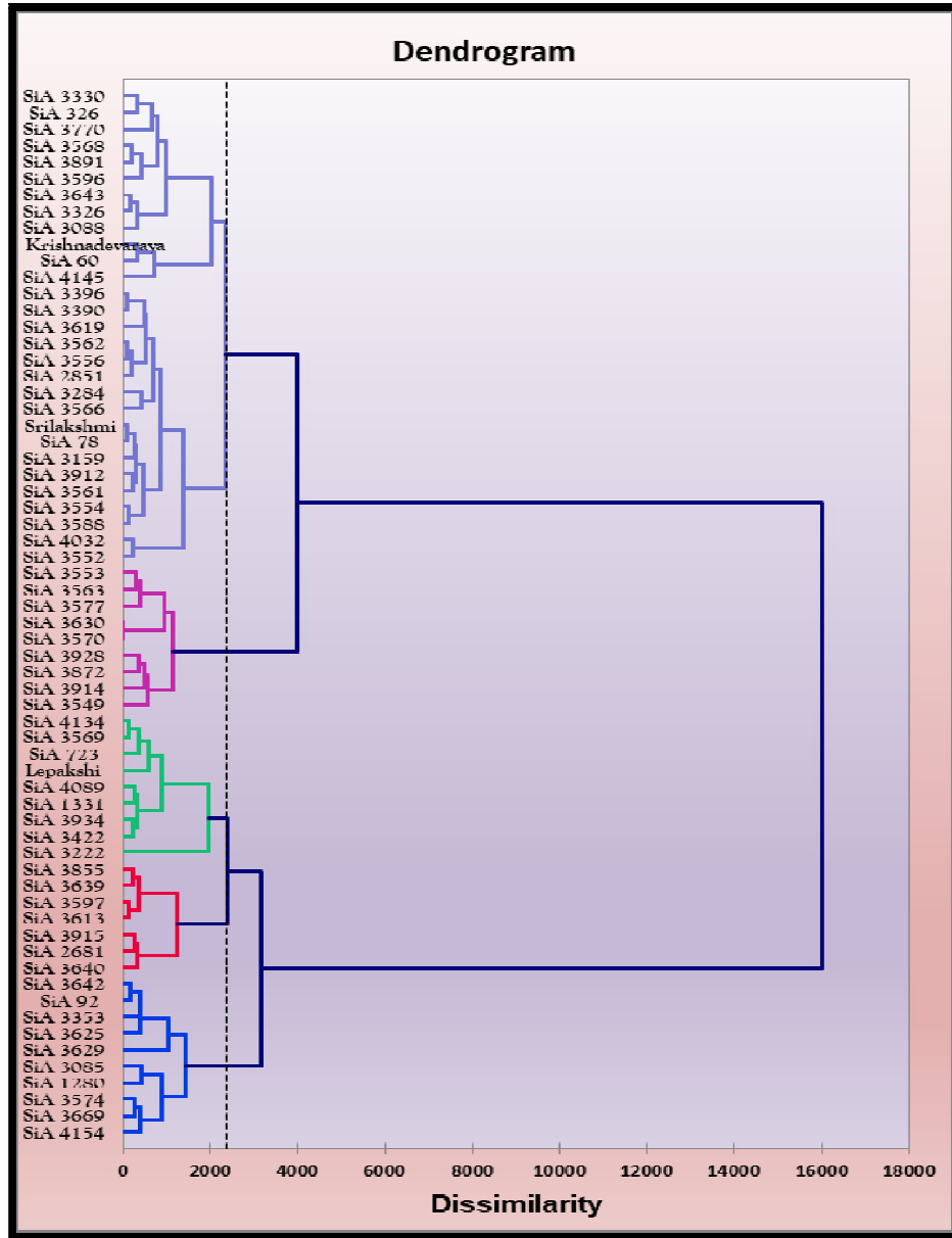
Fig. 3. Dendrogram showing relationship in five clusters based on Euclidean 2 distance in 64 genotypes of foxtail millet ( Setaria italica (L.) Beauv.)
