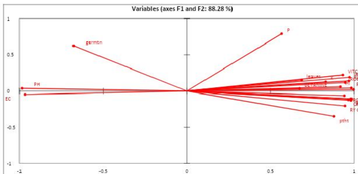
Figure 1: Biplot graphic with two principal components (PC1 and PC2: 88.28 %) for 21 parameters in beet root grown under alkaline conditions.
