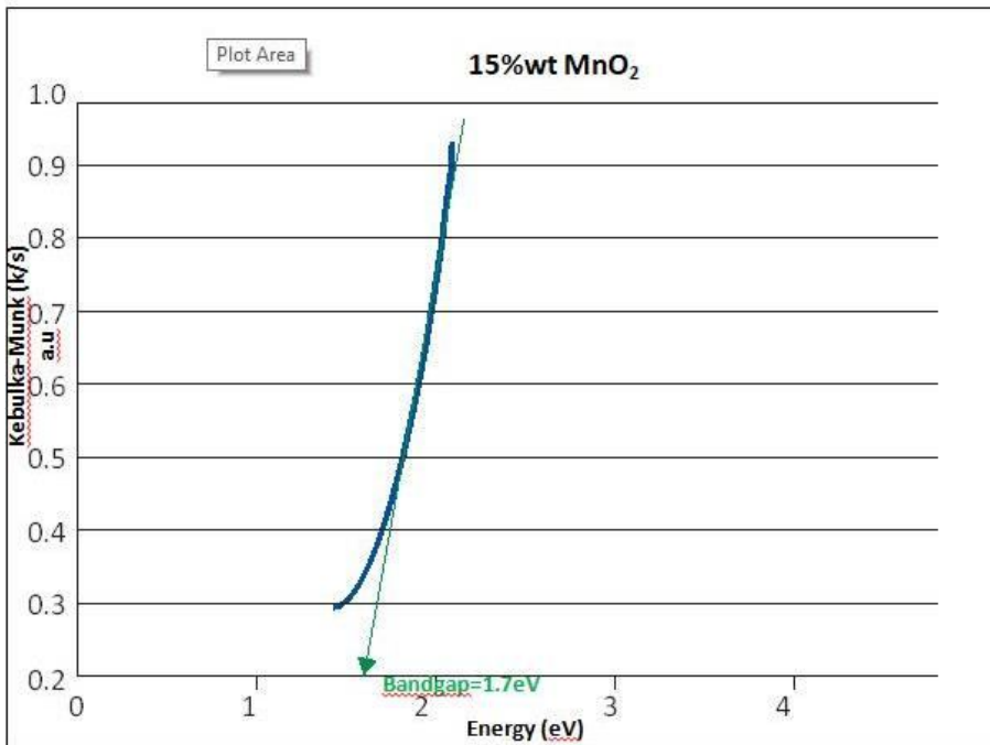
Fig. 4: Estimation of band gap value of TiO 2 doped with 15%wt MnO 2 using kubelka-munk plot
