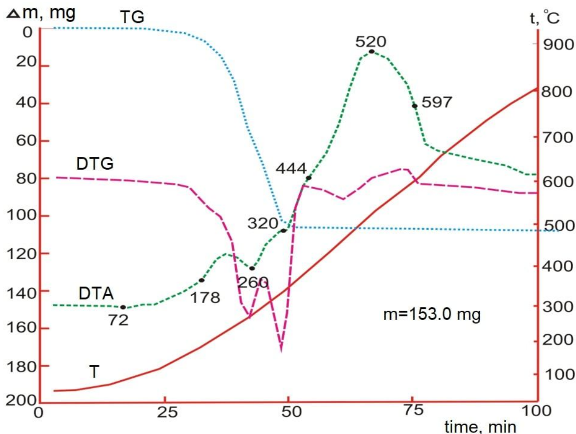
Fig.2. Derivatogram of Cu(NA-H) 2 ·2AA·2TC
