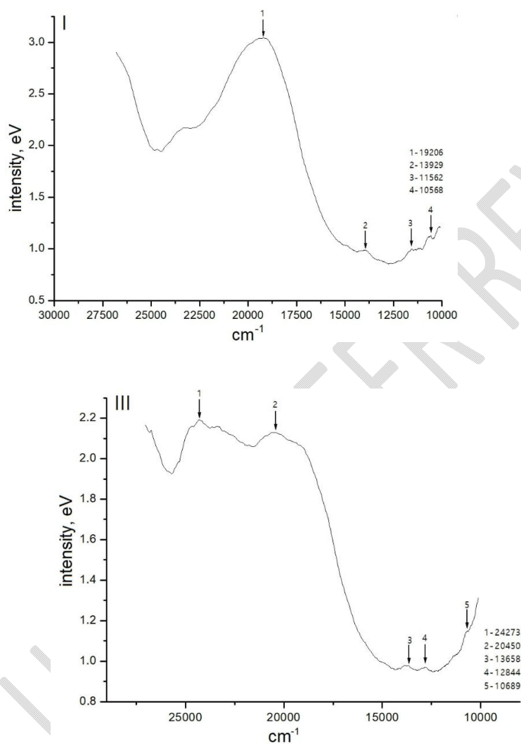
Fig.3. EDRS: I - \text{Cu}(\text{NA-H})_2 \cdot 2\text{AA} \cdot 2\text{TC} , II - \text{Cu}(\text{NA-H})_2 \cdot 2\text{C} \cdot 2\text{NAM} ; III - \text{Cu}(\text{NA-H})_2 \cdot 2\text{TC} \cdot 2\text{NAM} .
