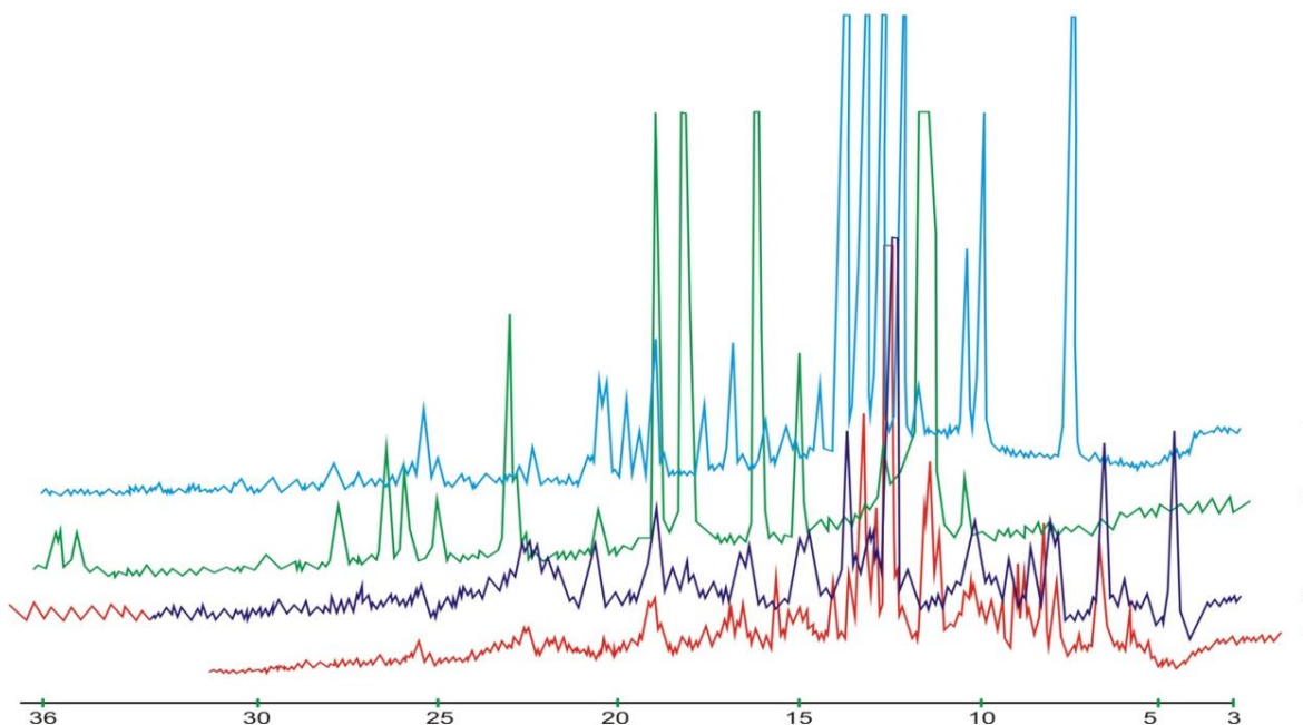
Fig. 1. X-ray diffraction patterns of \text{NC}_5\text{H}_4\text{CONH}_2 (1), \text{CO}(\text{NH}_2)_2 (2), \text{Cu}(\text{NC}_5\text{H}_4\text{COO})_2 \cdot \text{H}_2\text{O} (3), \text{Cu}(\text{NC}_5\text{H}_4\text{COO})_2 \cdot 2\text{CO}(\text{NH}_2)_2 \cdot 2\text{NC}_5\text{H}_4\text{CONH}_2 (4)
