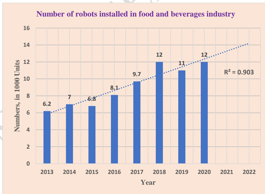
Figure 3. Worldwide number of robots installed in food and beverages industry in 2020 [2].
