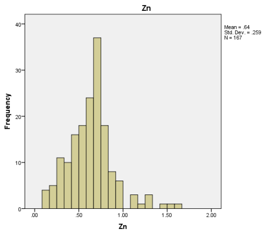
Figure 3. Frequency distribution of Zn (a), Cu (b), Fe (c), Mn (d), and B (e) of Kishtwar soils
