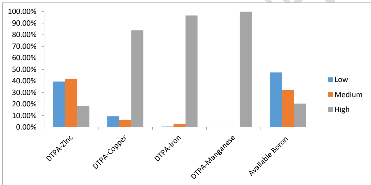
Figure 4. Percentage distribution of different micronutrient categories in soils of Kishtwar district
