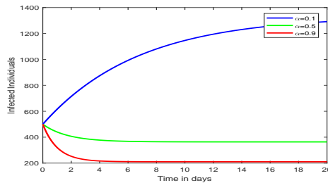
Figure 3: Impact of Vaccination on reducing infections in age group 1
