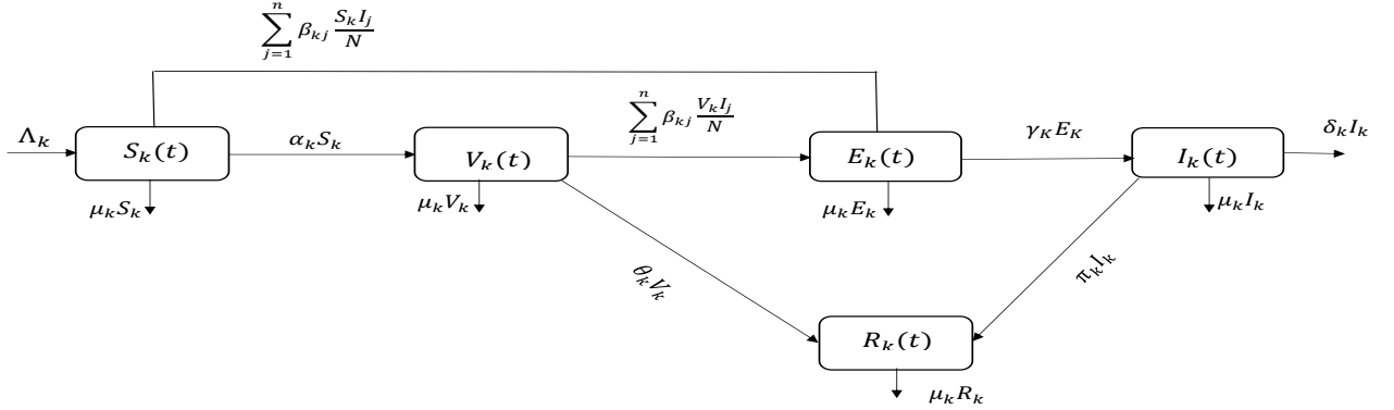
Figure 1: Discrete Age Structured Model flow diagram
