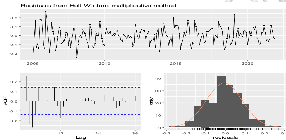
Figure 10. Model adequacy check for Holt-Winters' multiplicative model
