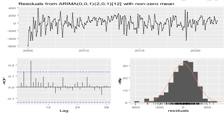
Figure 8. Model adequacy check for ARIMA (0,0,1) (2,0,1) [12]
