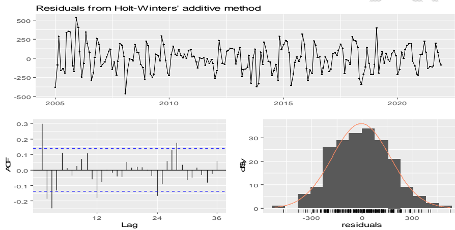
Figure 9. Model adequacy check for Holt-Winters' additive model
