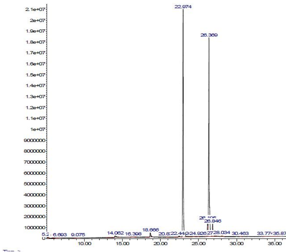
Fig. 2. GC-MS analysis of A. grandiflora
