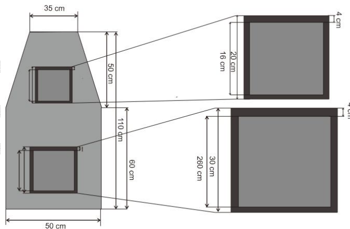
Fig 6. Pyrolysis Reactor
