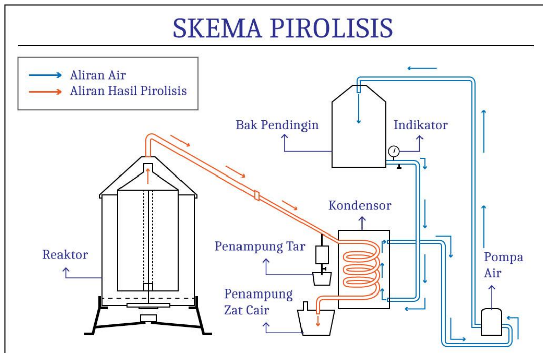
Fig 2. Pyrolysis Scheme
