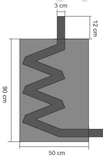
Fig 8. Condenser
