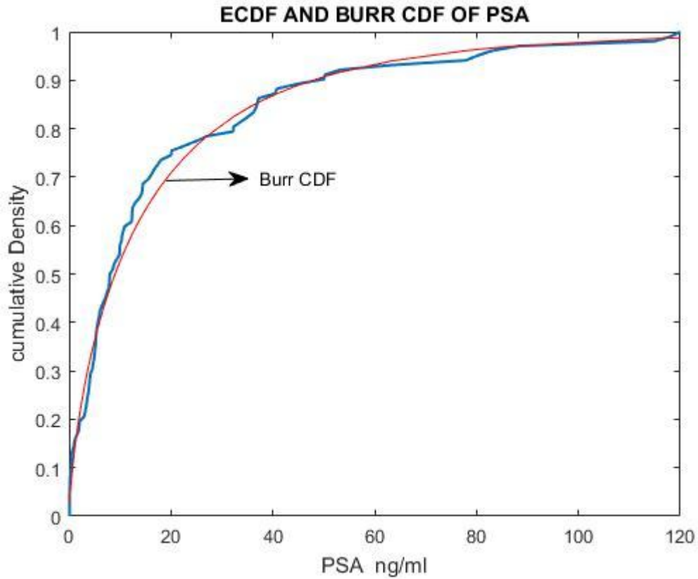
Fig. 3 shows that the Burr distribution is a very good fit to the empirical distribution of the PSA data. It can also be observed that the Burr distribution may give slightly different cumulative densities when the PSA values fall between 20.0ng/ml and 40.0ng/ml.
