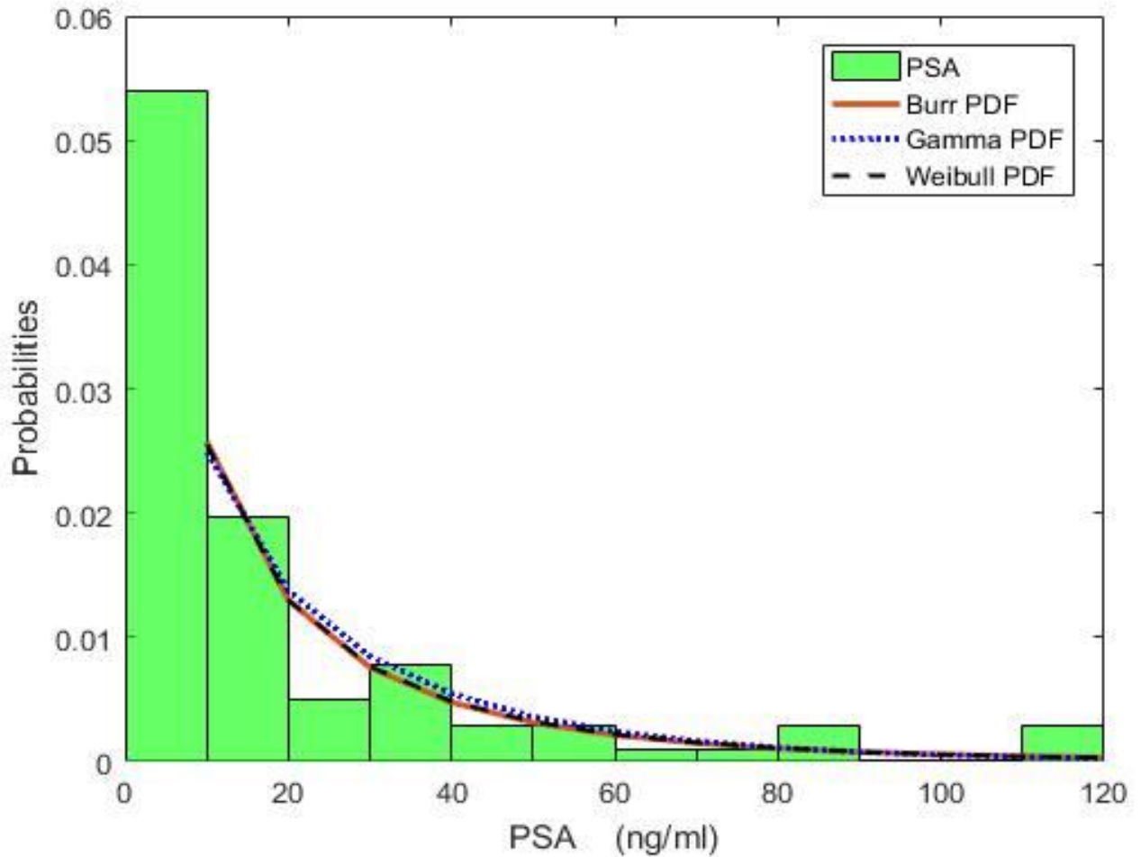
Figure 4.2 shows that the Weibull and Burr distributions seem to fit the data better than the Gamma distribution.
