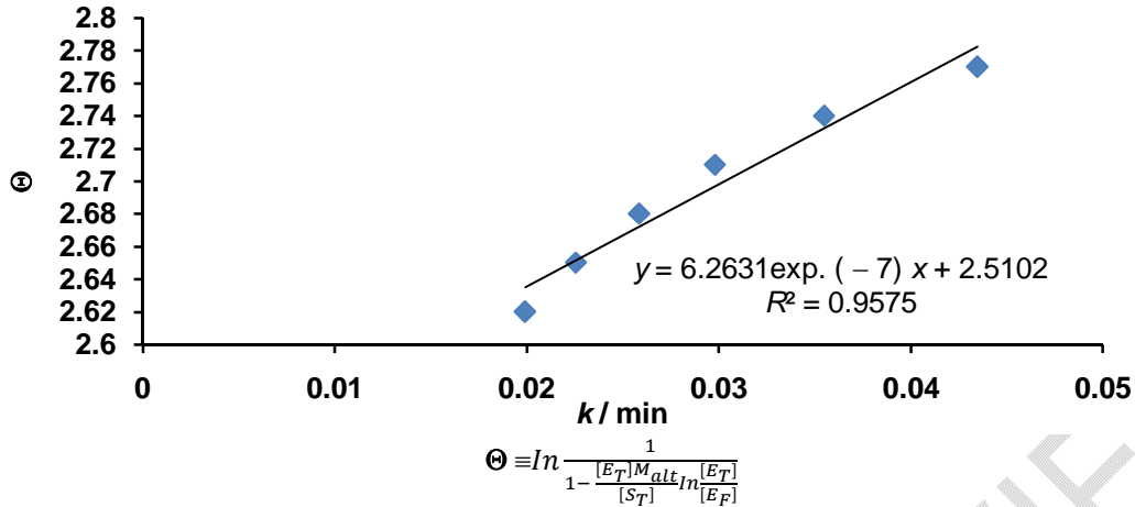
Fig. 1: Determination of the duration, t_{ES} , of ES formation for [S_T] \gg [E_T].M_{alt} , [E_T] and [S_T] , and [E_F] are molar mass of maltose, total concentrations of enzyme and substrate, and concentration of free enzyme respectively.
