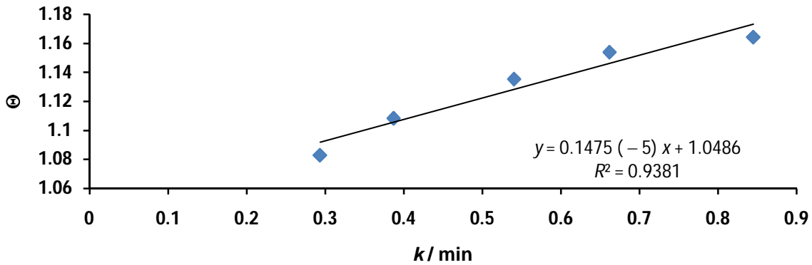
Fig. 2b: Determination of the duration, t_{ES} , of ES formation, for [S_T] \ll [E_T] . Definition of symbols, are as in Fig. 1. The range of [S_T] used for the plot is 1.2 \rightarrow 3 g/L. The full range, 0.3 \rightarrow 3 g/L showed poor correlation = 0.8116 ( R^2 = 0.6587 ) for what was a hyperbolic curve Fig. is not shown.
