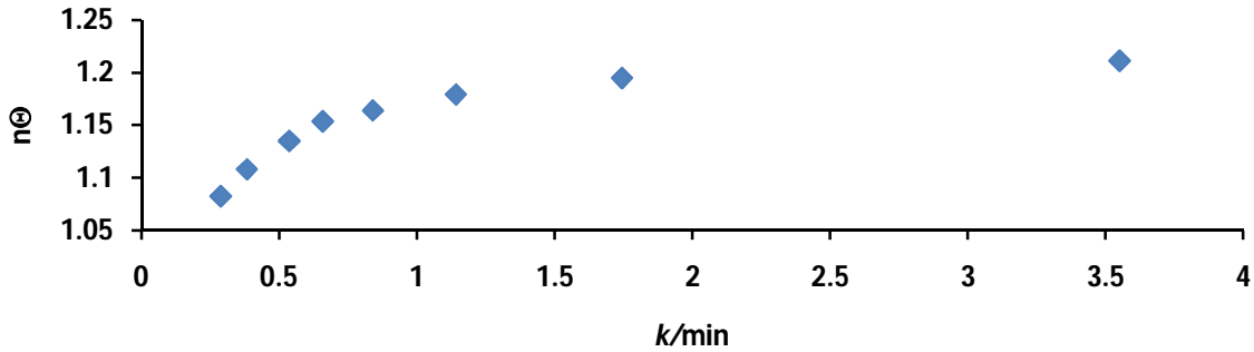
Fig. 2a. Plot showing nonlinear curve for the complete substrate concentration range for the determination of t_{ES} . A better coefficient of determination is applicable in the range 1.2 → 3 g/L. \Theta is defined in Fig. 1.
