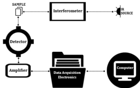
Fig 2. Working Principle of the Fourier Transform Infrared Source: Munajad et al. [13]
