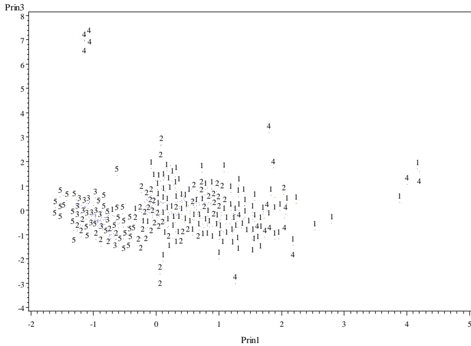
Fig.2 Principal component analysis of all Indian Fresh water species of Family Schilbeidae
