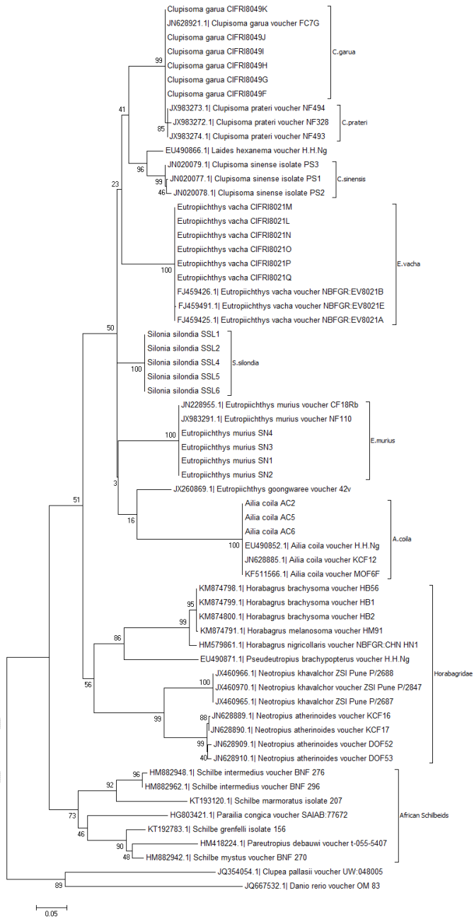
Fig 3 Evolutionary relationships of taxa
