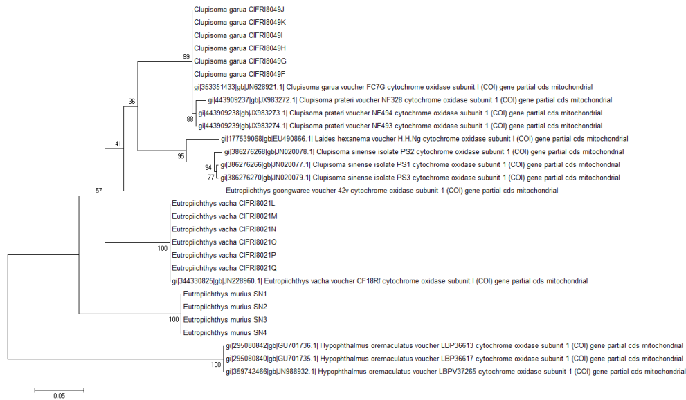
Fig 4 Molecular Phylogenetic analysis by Maximum Likelihood method
