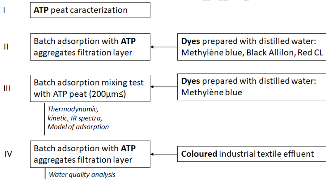
Fig. 1. Methodology diagram chart for the study of the use of allochthonous peat in dyes removal
