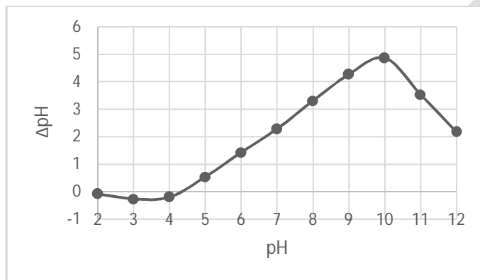
Fig. 2.3. Curve for the zero charge point determination of ATP
