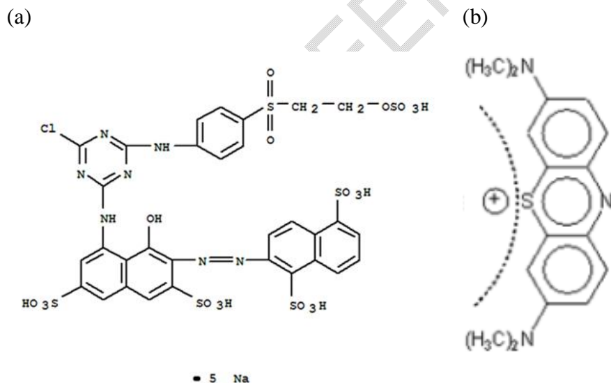
Fig. 4.2. Chemical structures of dyes RCL (a) [8] and BLM (b) [9]
