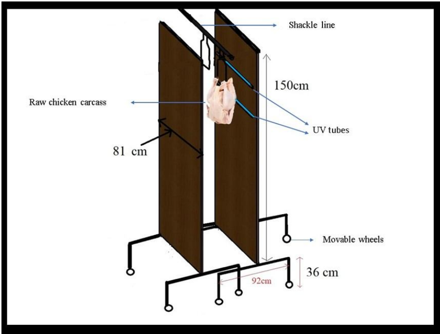
Fig 1: Ultraviolet-C (UV-C) chamber prototype device
