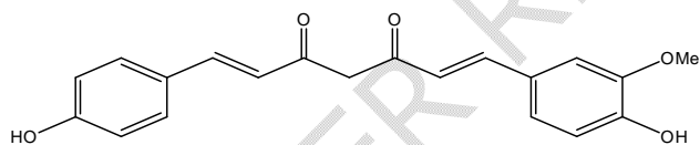
demethoxycurcumin
