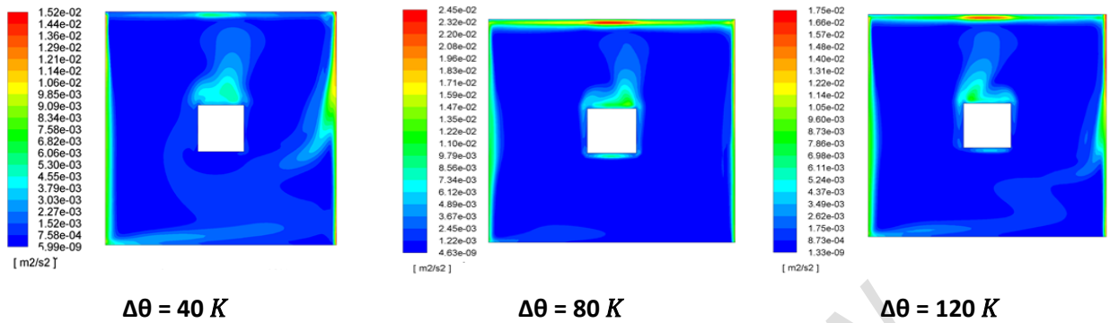
Figure 11: Isovalues of the turbulent kinetic energy for different values thermal gradient
