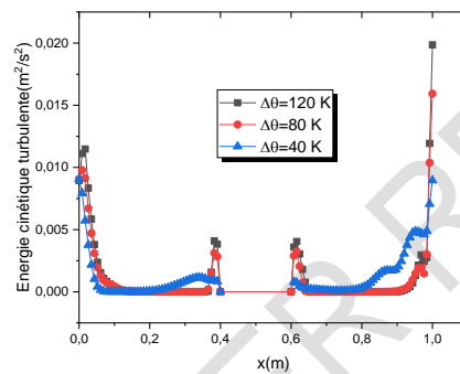
Figure 12: Profiles of the turbulent kinetic energy as a function of x for different values of the thermal gradient
