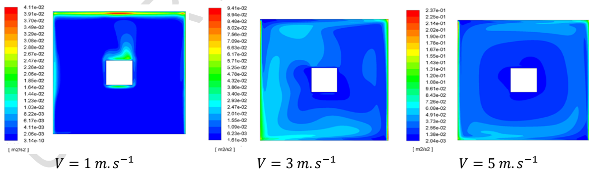
Figure 19: Isovalues of the turbulent kinetic energy for different values of the wall velocity
