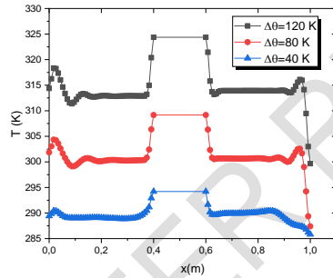
Figure 10: Temperature profiles as a function of x for different values of the thermal gradient
