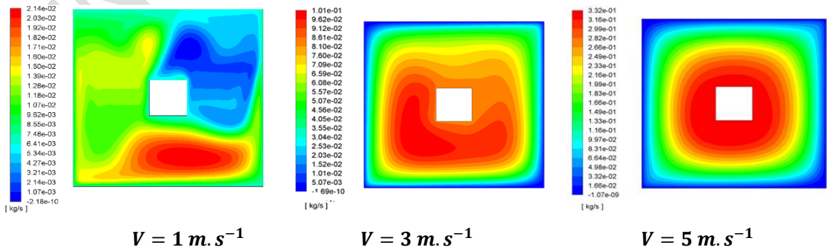
Figure 15: Streamlines for different values of wall speed
