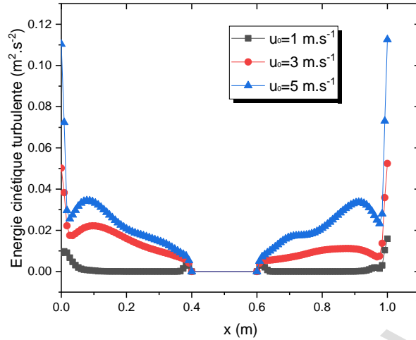
Figure 20: Profiles of turbulent kinetic energy as a function of x for different values of the modulus of the velocity of vertical walls in opposite directions
