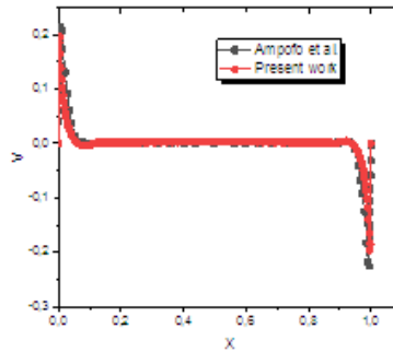
Figure 2: Comparison of v velocity at y = 0.5
