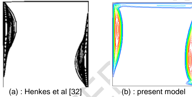
Figure 6: Comparison of contour plot of turbulent viscosity
