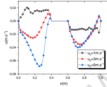
(b): u velocity profile
