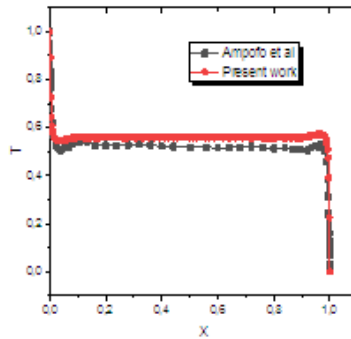
Figure 3: Comparison of temperature at y = 0.5
