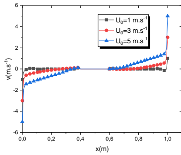
(a): v velocity profile
