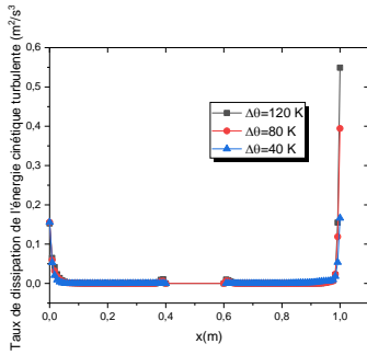
Figure 14: Profiles of the turbulent kinetic energy dissipation rate as a function of x for different values of the thermal gradient
