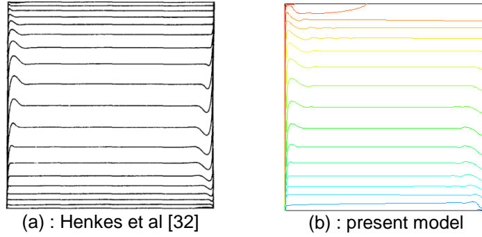
Figure 4: Comparison of streamlines
