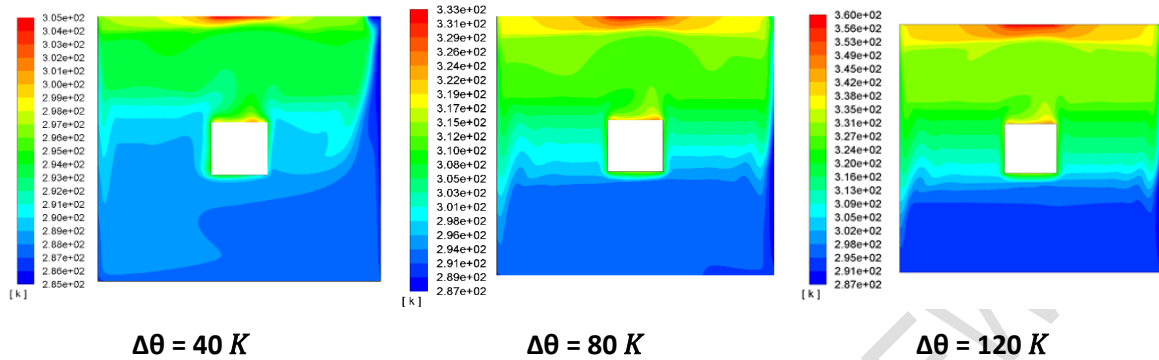
Figure 9: Isotherms for different values of the thermal gradient
