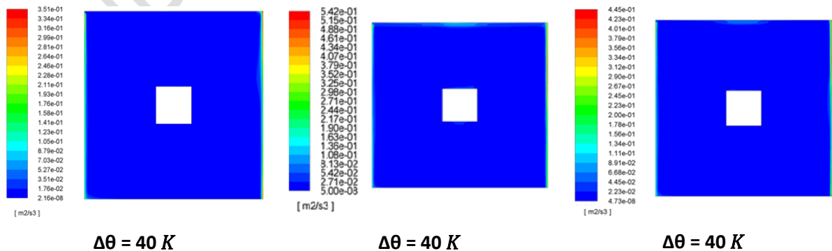
Figure 13: Isovalues of the turbulent kinetic energy dissipation rate for different values of the thermal gradient
