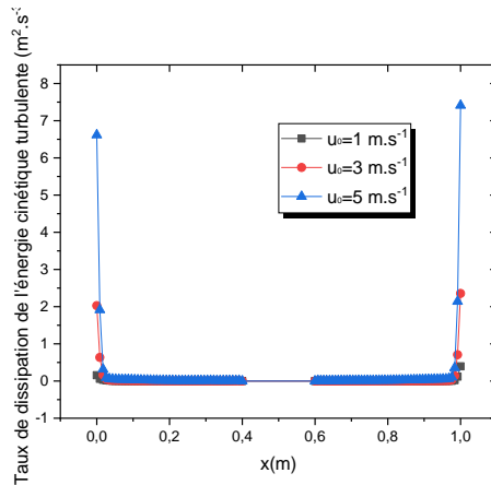
Figure 22: Profiles of turbulent kinetic energy dissipation rate as a function of x for different values of the modulus of the vertical wall velocity in opposite directions
