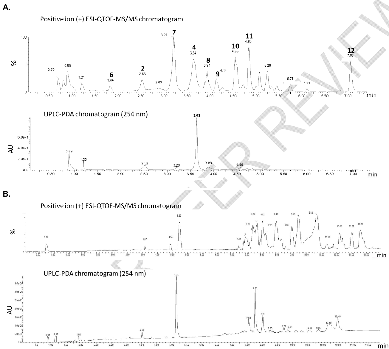
Figure 2. LC-MS/MS analysis of A. methanol and B. hexane extracts of Vitex negundo showing the positive ion (+) ESI-QTOF-MS/MS and UPLC-PDA chromatograms
