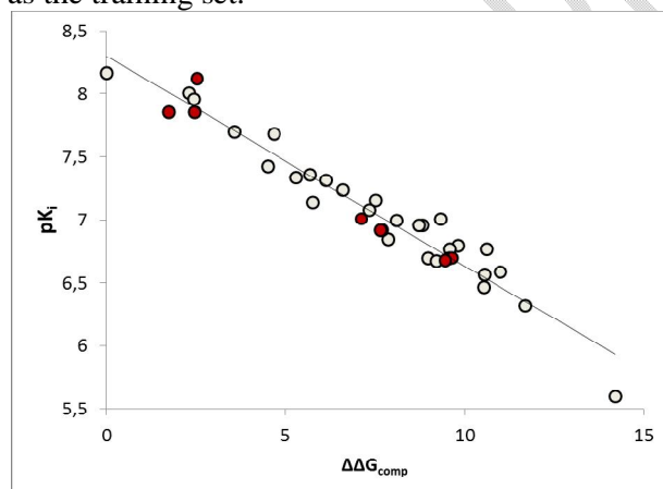
Figure 3. Plot for relative complexation Gibbs free energies of the PPO-CQBx complex formation \Delta\Delta G_{\text{com}} [ \text{kcal.mol}^{-1} ] of the training set [15]. The validation set data points are shown in red color.
