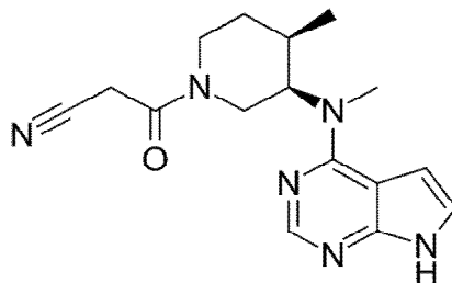
Figure 1. Chemical structure of Tofacitinib
