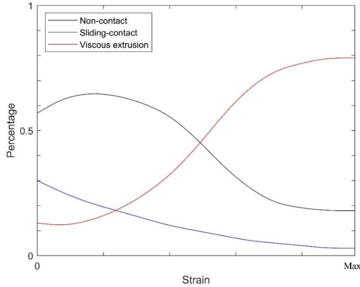
Fig.6. Proportion of contact states distribution in MR
