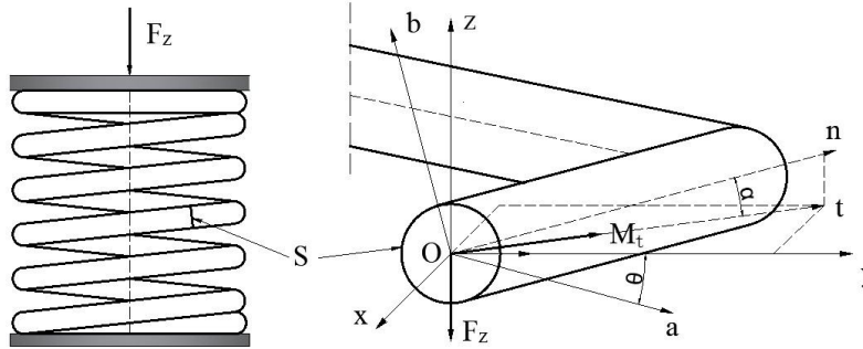
Fig.4. Analysis of axial loading on the micro-unit
