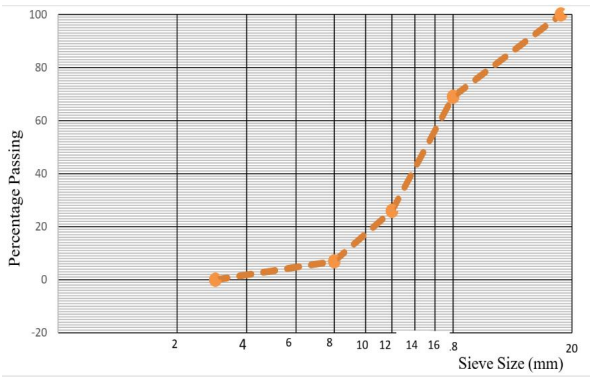
Fig 8: Particle size distribution of crushed granite
