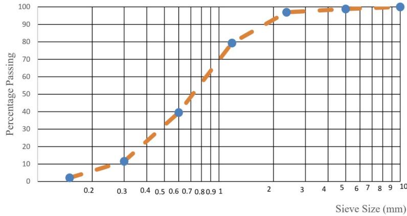
Fig 10: Particle size distribution curve for sand.
