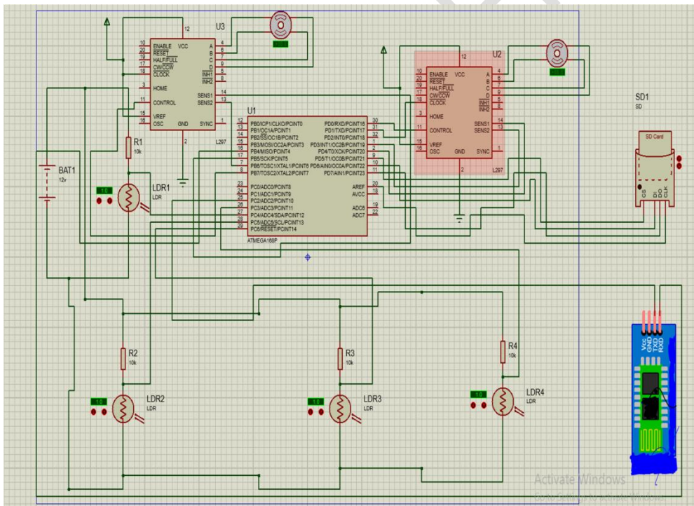
Fig. 1. The complete circuit diagram of the DASPGS
