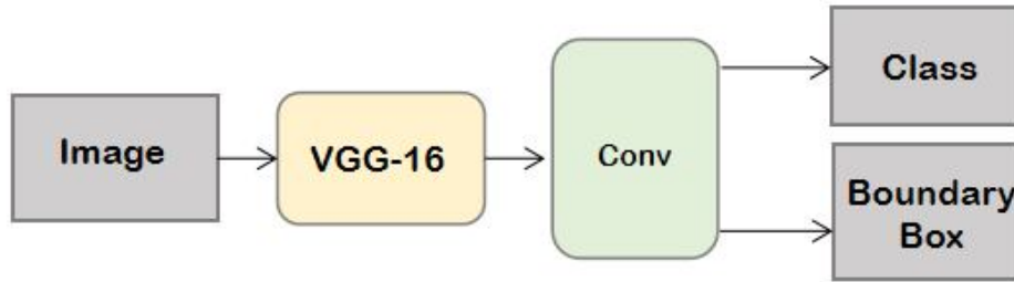
Figure 5: Architecture of SSD
