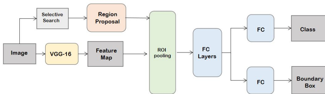
Figure 2: Architecture of Fast R-CNN
