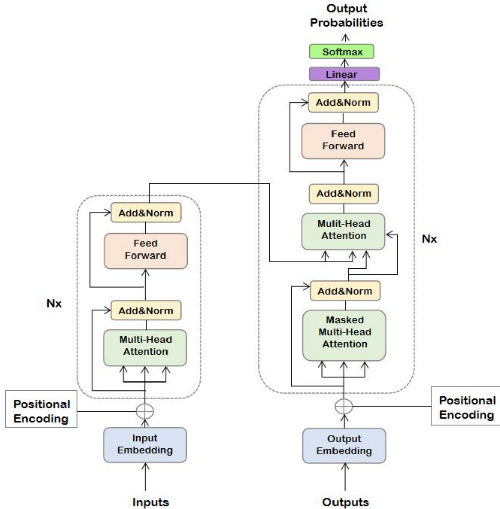
Figure 6: Architecture of Transformer
