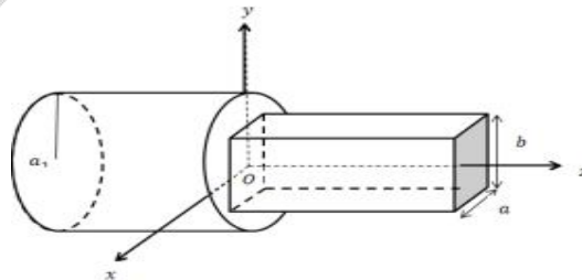
Figure 3 : Junction between a circular and a rectangular guide whose the surface of the rectangle being inferior than that of the circle.
