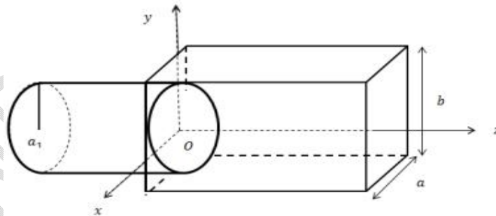
Figure 4 : Junction between a circular and a rectangular guide whose the surface of the rectangle being greater than that of the circle.
