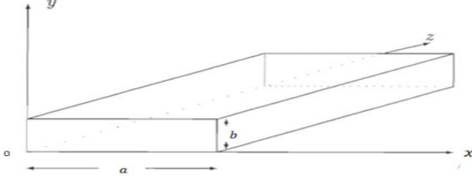
Figure 1: Right section of the rectangular waveguide
