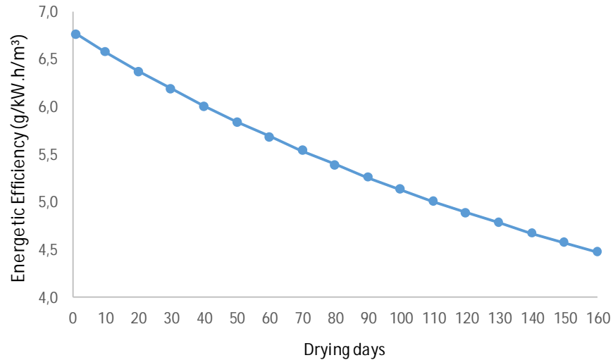
Fig. 2. Relationship between wood drying time (days) and transport energetic efficiency (g/kW.h/m 3 ), under the study conditions
