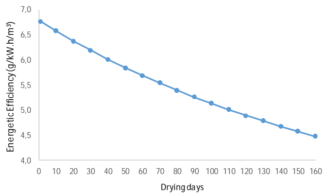
Fig. 2. Relationship between wood drying time (days) and transport energetic efficiency (g/kW.h/m 3 ), under the study conditions
