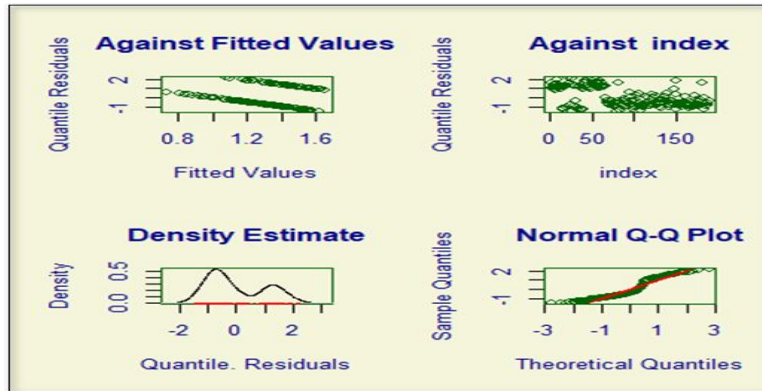
Figure 1. Graphical test for nonlinearity, outliers and homoscedasticity
