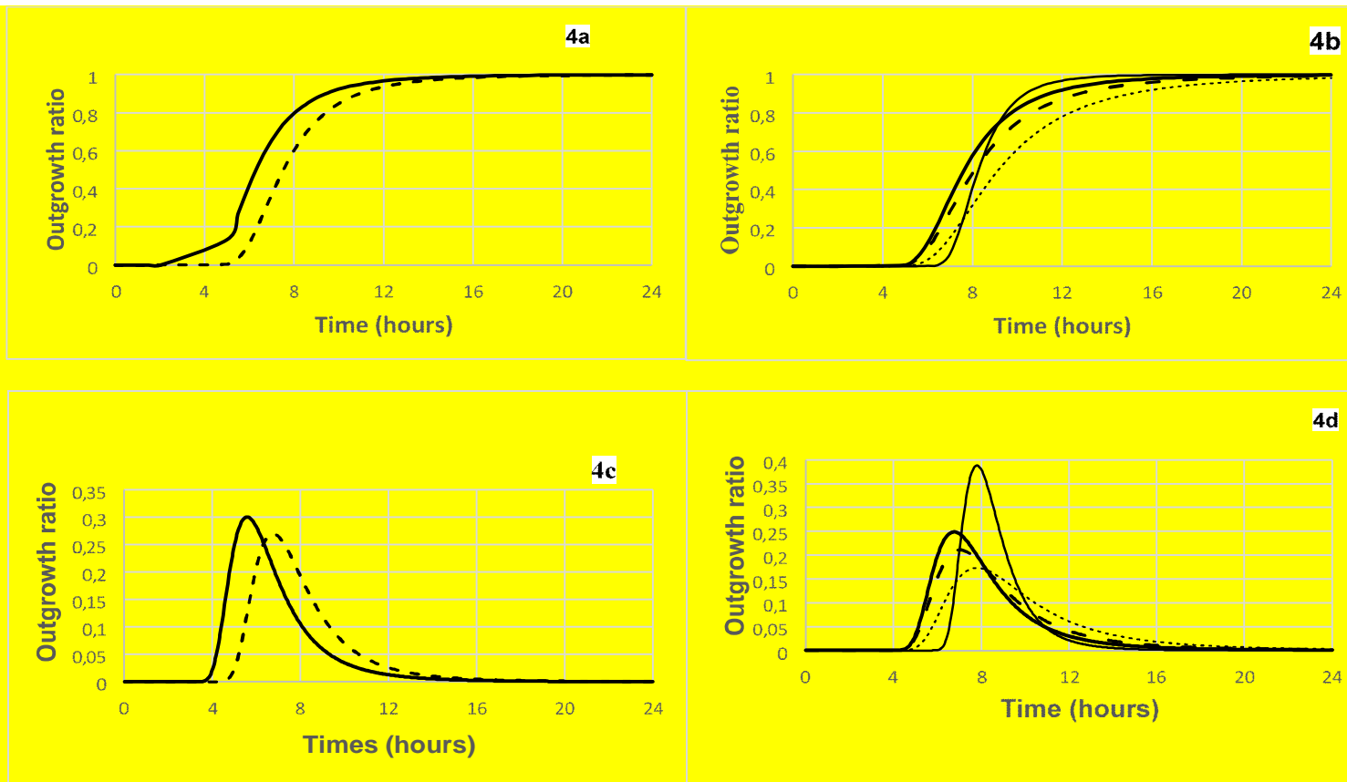
Figure 4: Outgrowth(a) and mode (c) of the distribution of times for the first colony to emerge from B. cereus spore (solid line) and B. subtilis spores produced in the same medium and heat activated. Example of outgrowth (b) and mode (d) of B. cereus spores (solid interrupted line) and B. subtilis spores (thin interrupted line) produced in the medium contained 60g, 12.5g and 2.5g/L; and for B. cereus spores (solid line) and B. subtilis (thin line) produced in a medium contained 60g, 37.5g and 2.5g of carbohydrates, lipids and proteins respectively (b and d).
